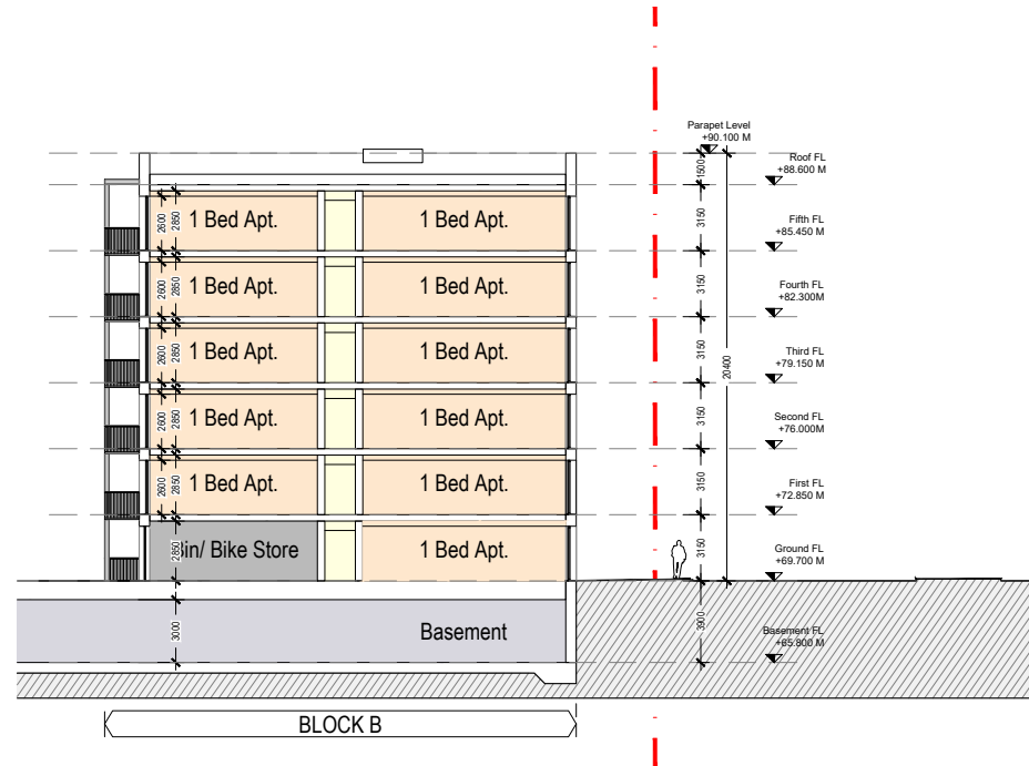
Block B - Section BB
