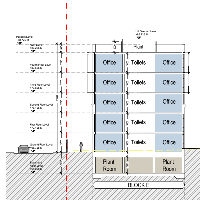
Block E - Section EE
