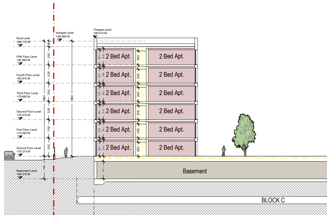
Block C - Section CC
