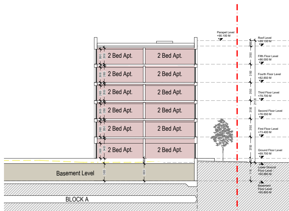
Block A - Section AA
