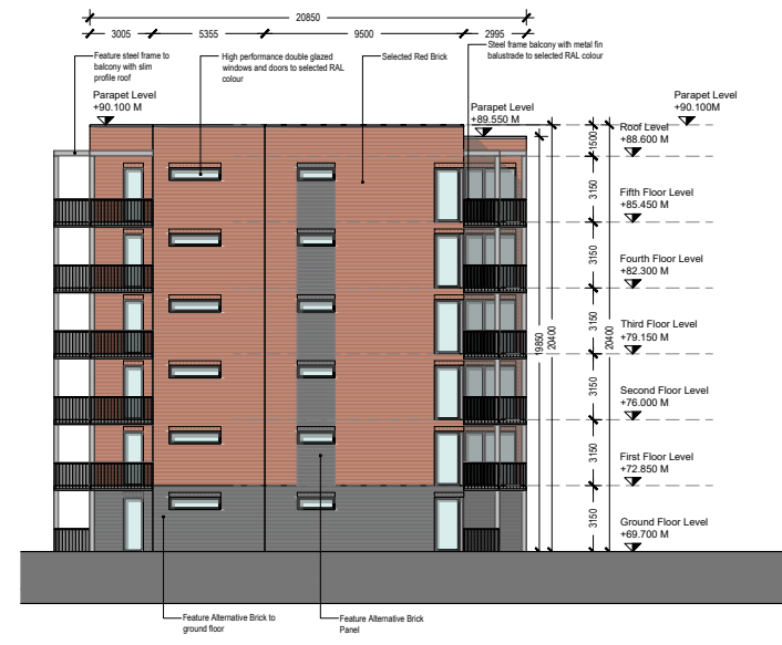
Northern Elevation
