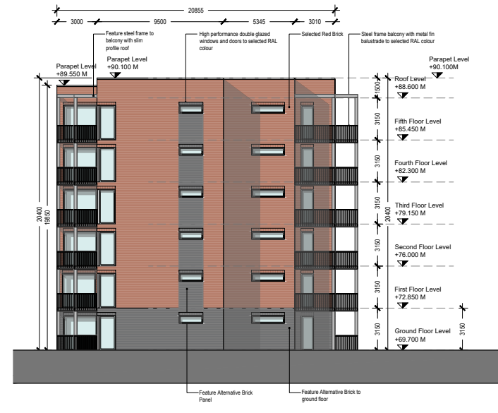
Southern Elevation
